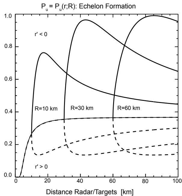
Fig. 2.2. Effect of the underlying sensor-to-group geometry: resolution probability depending on the distance between group center and radar for R = 0, 10, 30, 60 km.
